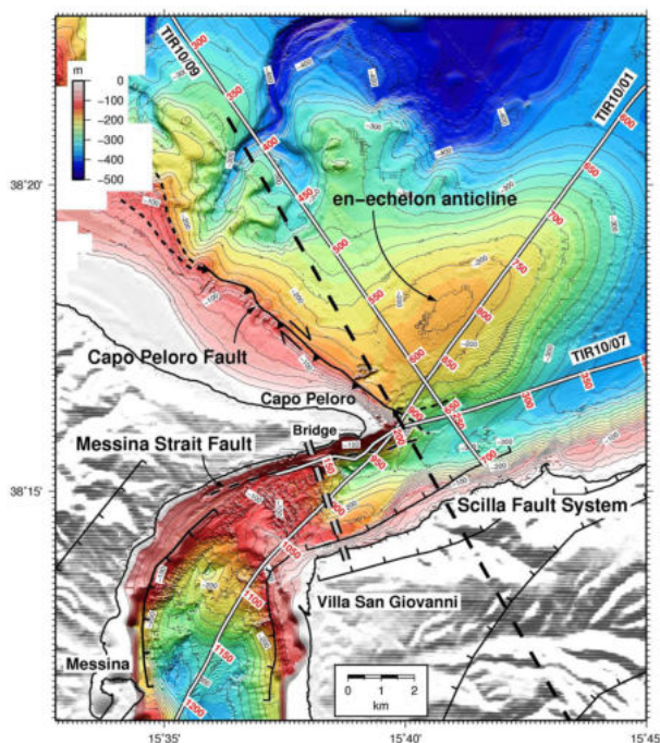
Fig. 25 - Mappa dell’area dello Stretto, tratta dall’articolo “The tectonic puzzle of the Messina area (Southern Italy): Insights from new seismic reflection data” , di Doglioni et al. (2012).
